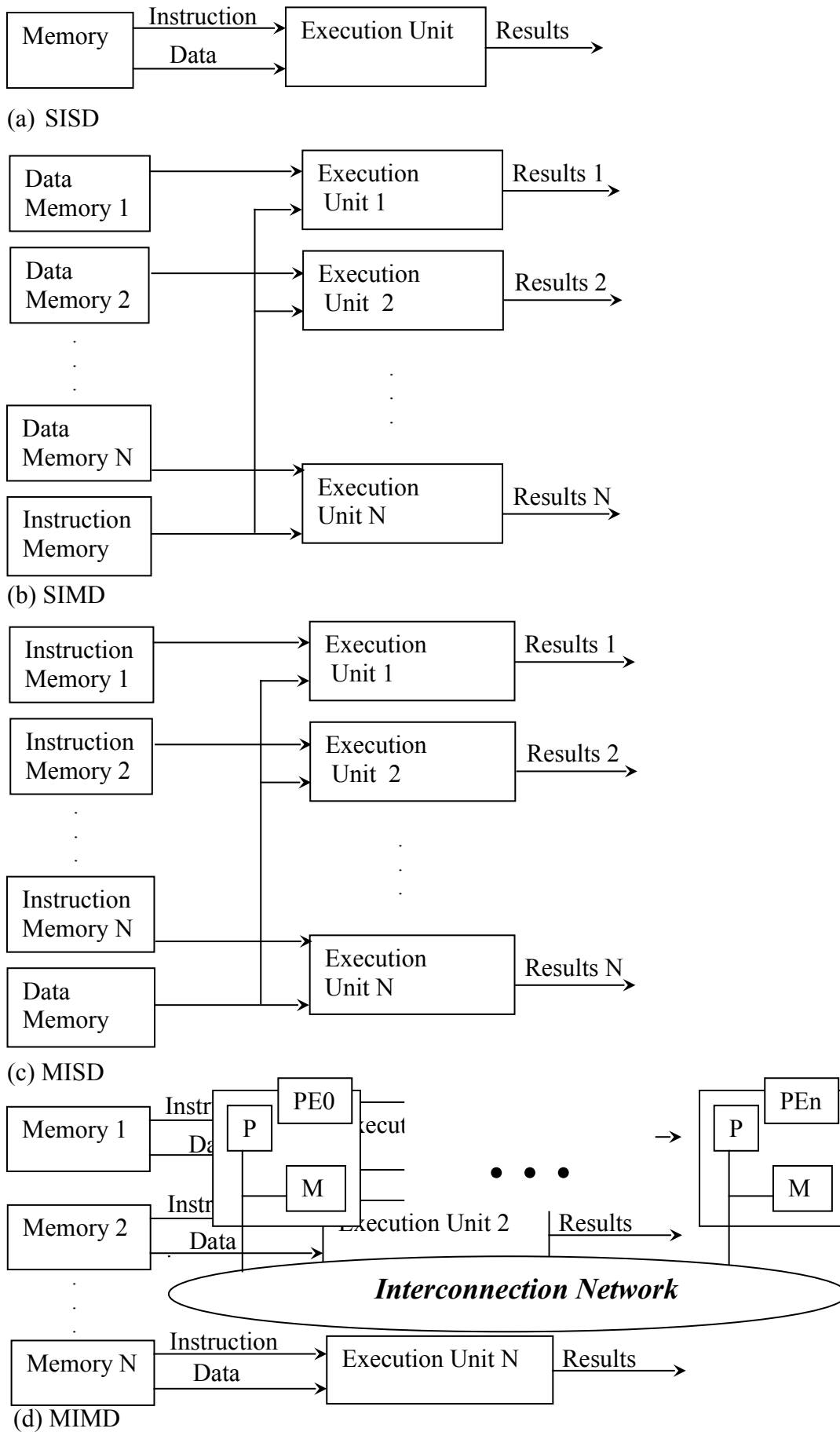
Fig.1.1. Classification of Flynn
